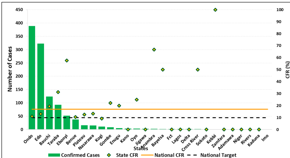
Figure 5: Number of confirmed cases with case fatality rate (CFR) by state week 43, 2023
