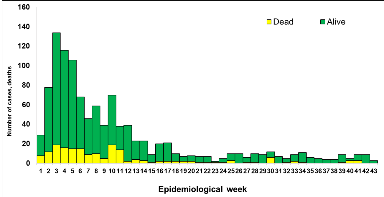
Figure 1. Confirmed Lassa fever cases in Nigeria epidemiological week 1, 2023 to week 43, 2023
