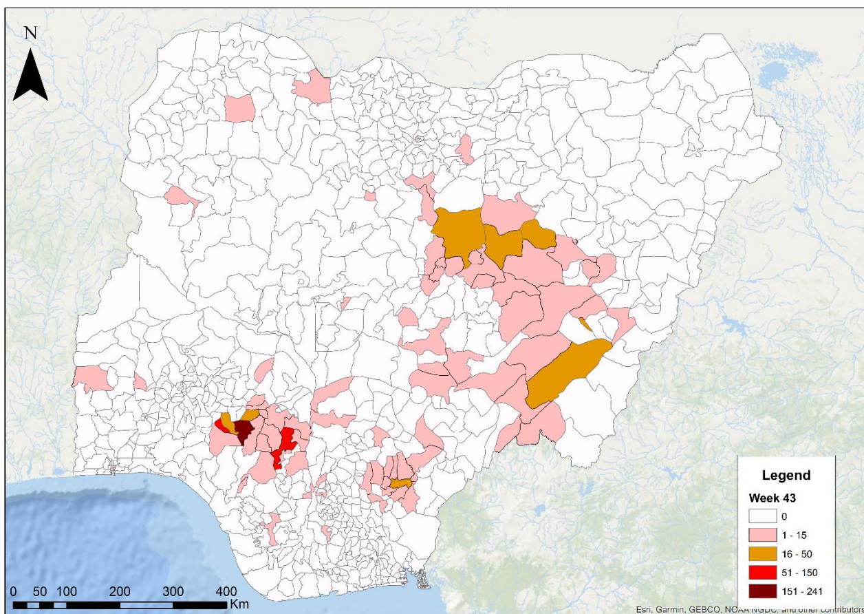
Figure 3. Confirmed Lassa fever rate per 100,000 population for LGAs in Nigeria, week 43, 2023
