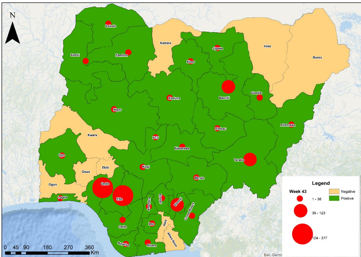
Figure 2. Confirmed Lassa fever cases by States in Nigeria, week 43, 2023
