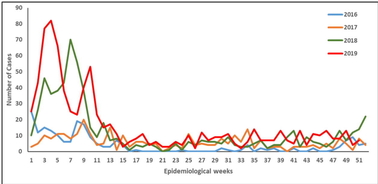
Figure 4. Weekly trends of Lassa fever Confirmed Cases in Nigeria, 2016/week 01-2019/week 52
