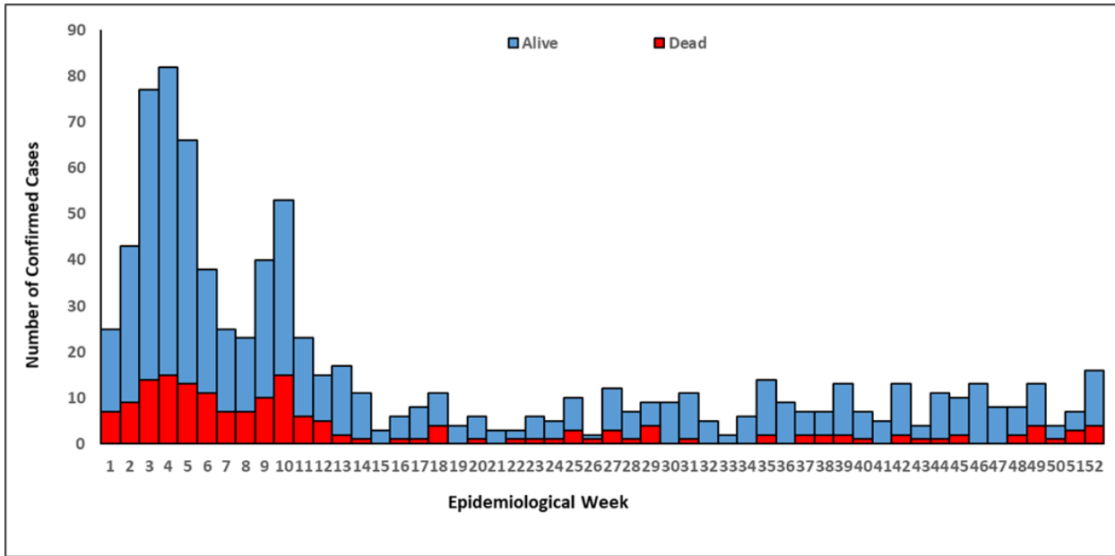
Figure 3. Epicurve of Lassa fever Confirmed Cases (833) in Nigeria - week 01-52, 2019
